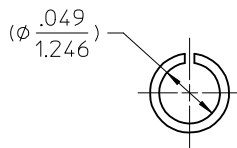
ALIGNMENT SLEEVE (ZIRCONIA CERAMIC)
