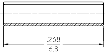
ALIGNMENT SLEEVE (ZIRCONIA CERAMIC)
