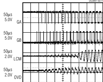
HALF-BRIDGE SOFT-START AT V_{INV} = 12.5V
