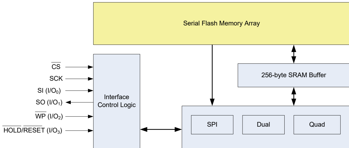
Figure 2. Block Diagram
