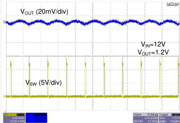
Figure 15. Static Output Ripple with No Load
