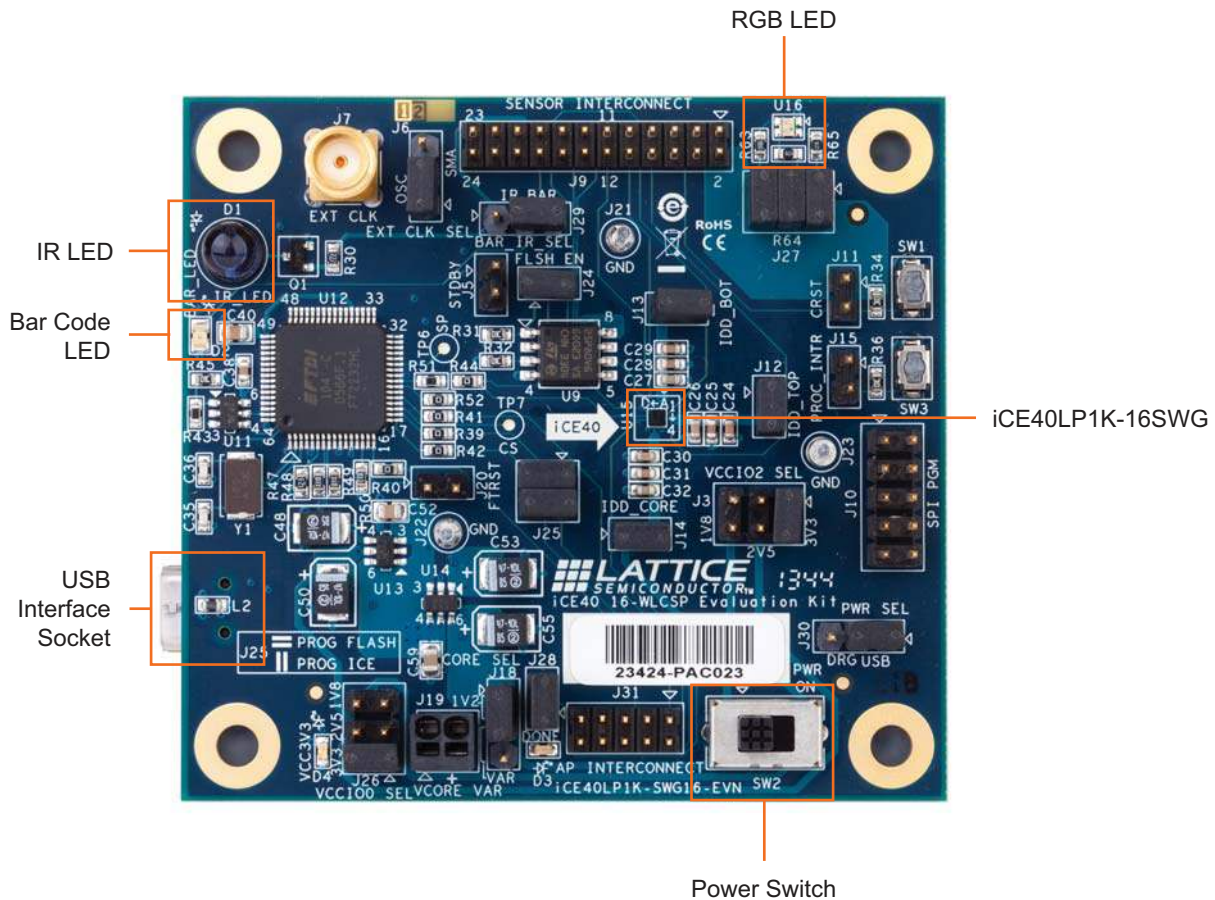
Figure 1. iCE40 16-WLCSP Evaluation Board (Top Side)
