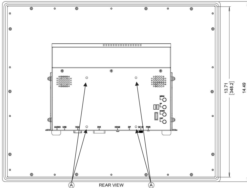
REAR VIEW
