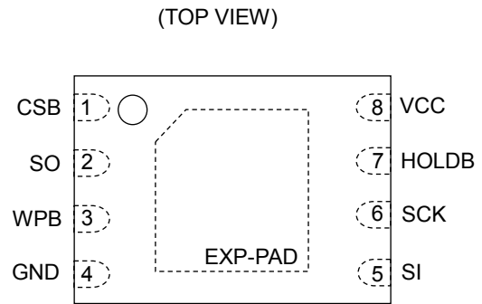
Figure 3-(b). Pin Configuration (VSON008X2030)
