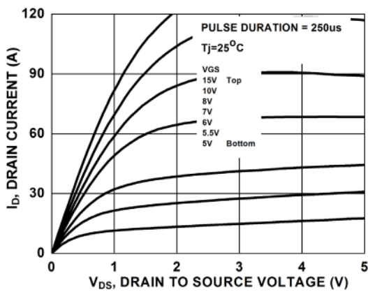
Figure 9. Saturation Characteristics
