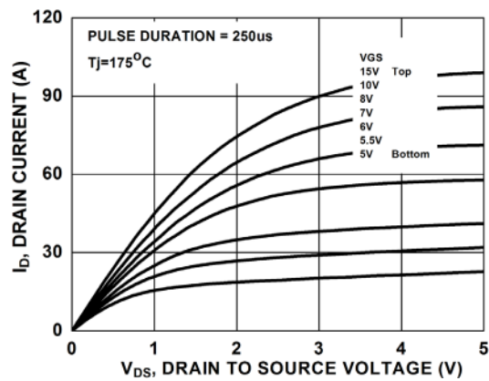
Figure 10. Saturation Characteristics
