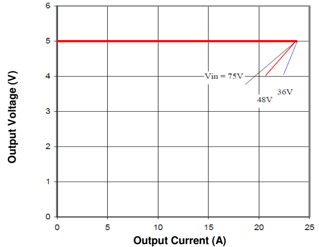
Figure 10. Output Characteristics
