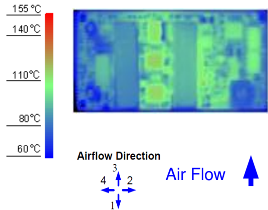
Figure 12. Thermal Image for Airflow Direction 3 (18.7A output, 55°C ambient, 200 LFM, typical V_{in} , open frame, socket interface)
