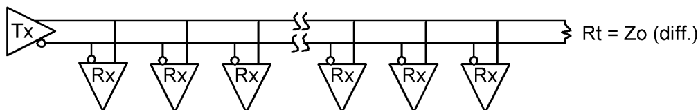
Figure 8. Multi-Drop Applications
