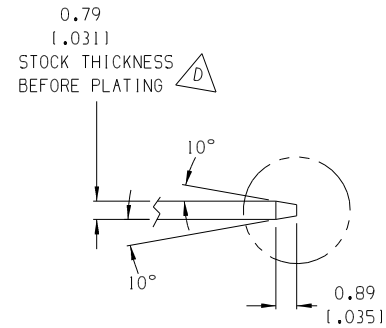
DETAIL "Z" SCALE 5:1
