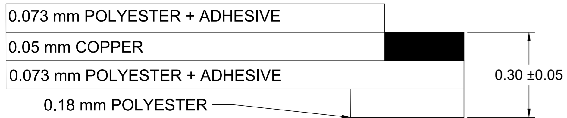
CROSS-SECTION
