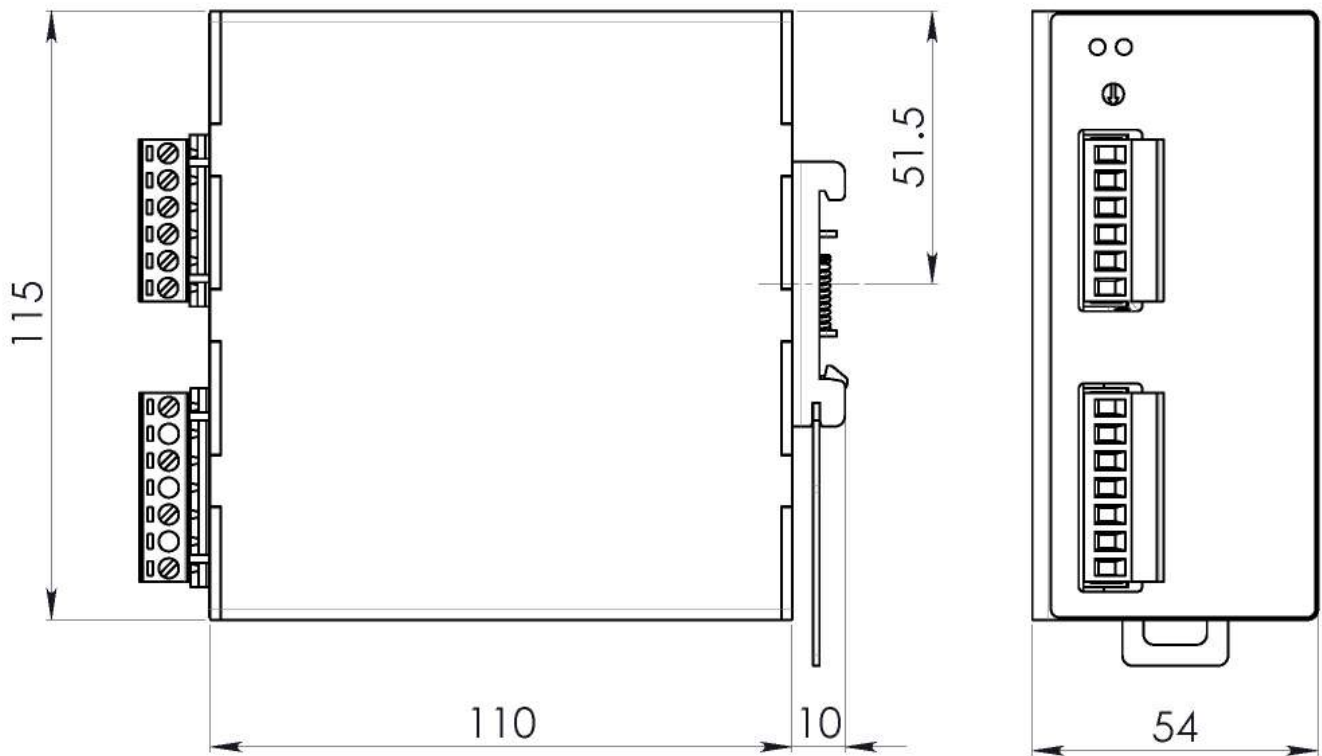
Figure 1. Mechanical Drawing
