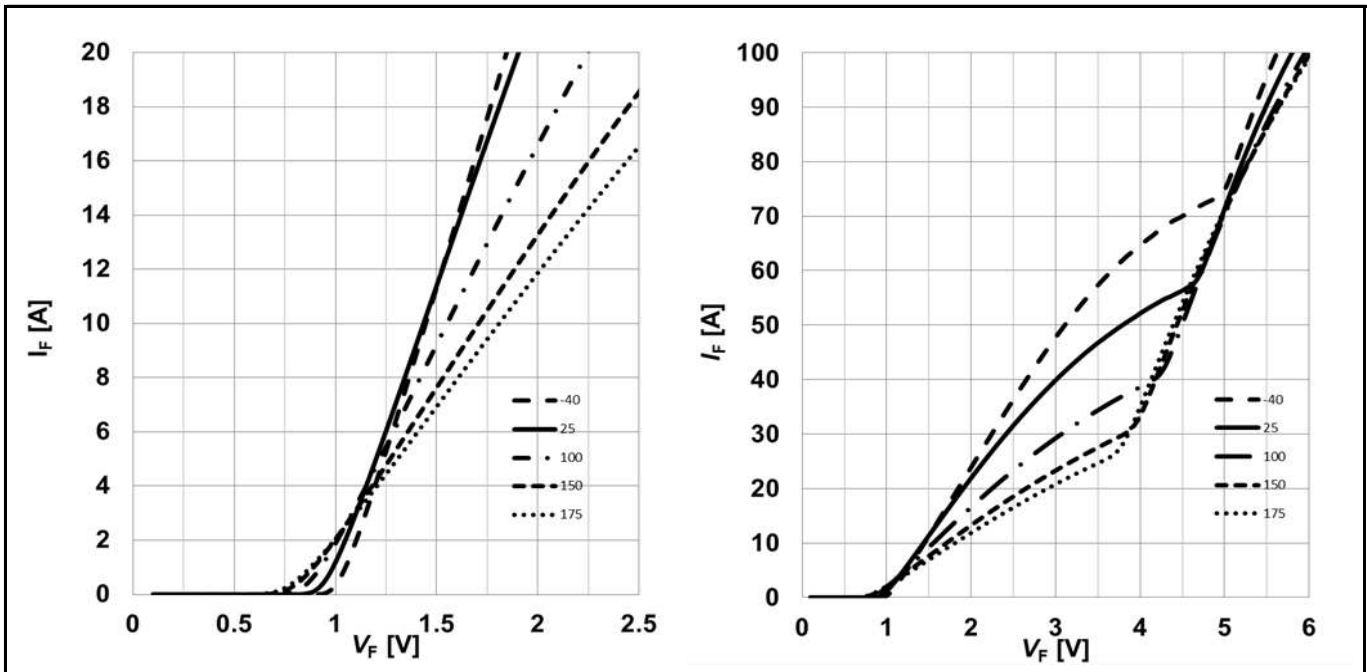
Figure 2 (LEFT) Typical forward characteristic; I_F = f(V_F) ; t_p=200\text{ }\mu\text{s} ; parameter: T_j (RIGHT) Typical forward characteristics in surge current; I_F = f(V_F) ; t_p=200\text{ }\mu\text{s} ; parameter: T_j
