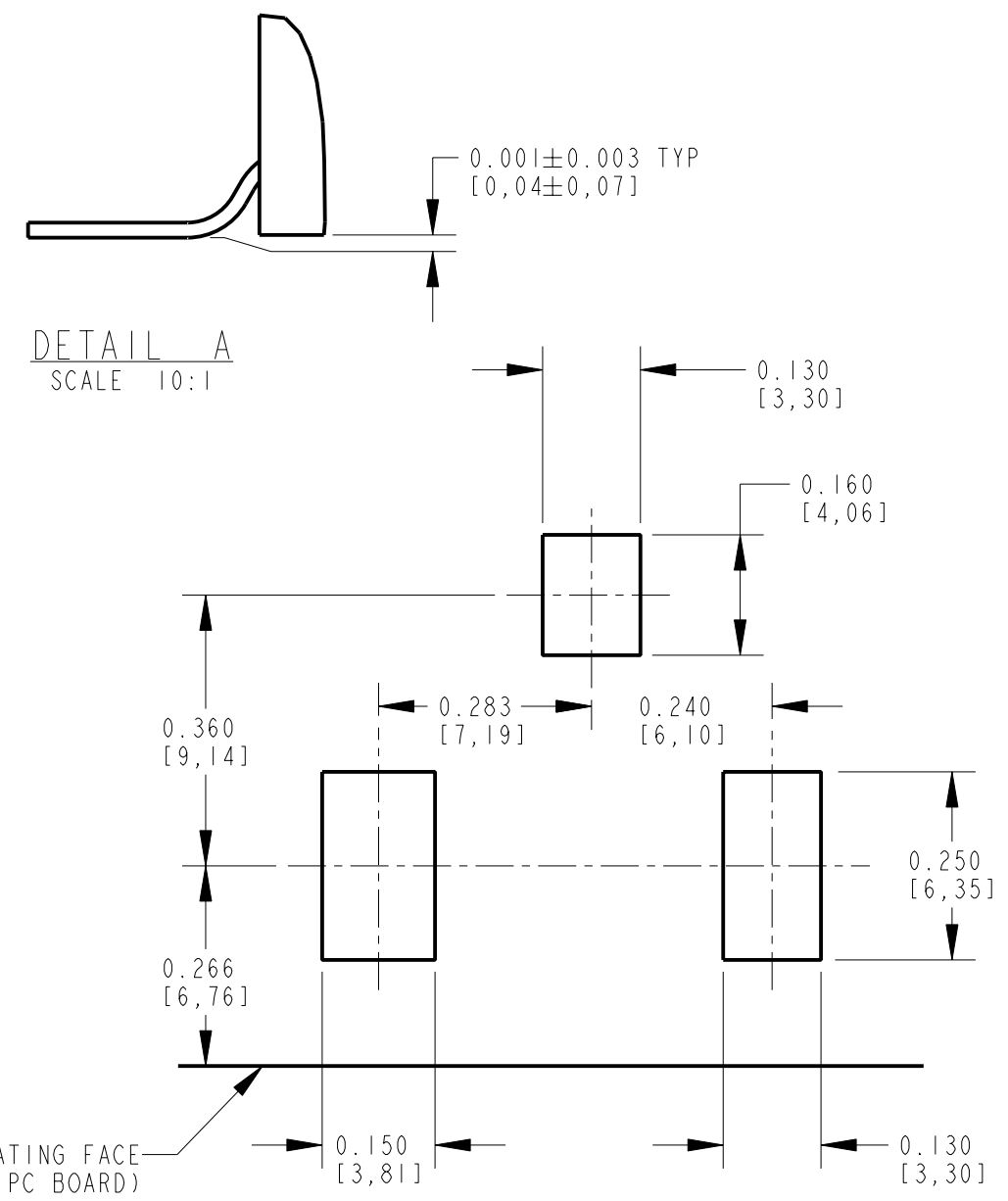
RECOMMENDED PC BOARD LAYOUT (COMPONENT SIDE)
