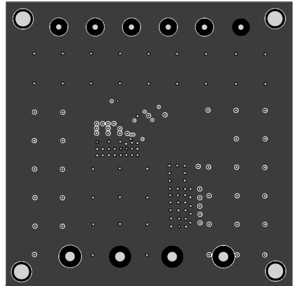
Figure 2: Inner Layer 1
