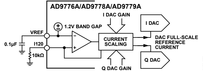
Figure 76. Reference Circuitry
