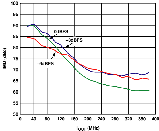
Figure 24. AD9779A IMD Performance vs. f_{OUT} , Digital Full-Scale Input Over Output Frequency, 4x Interpolation, f_{DATA} = 200 MSPS
