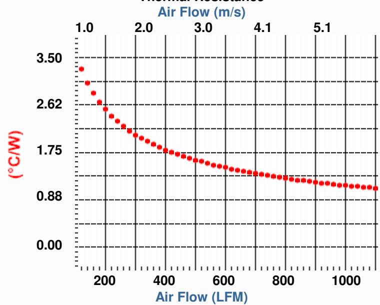
Heat Sink Thermal Resistance
