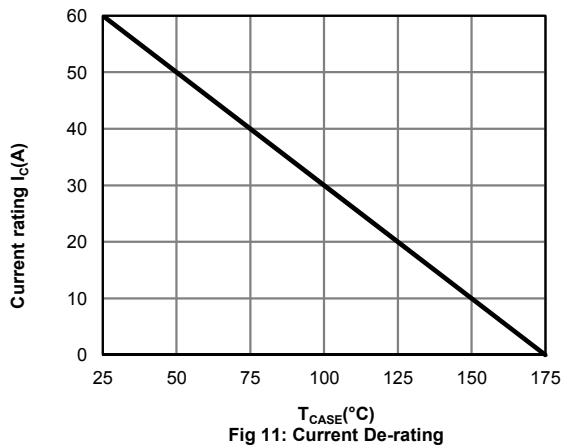
Fig 11: Current De-rating
