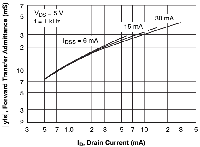
Figure 5. |y_{fs}| - I_D
