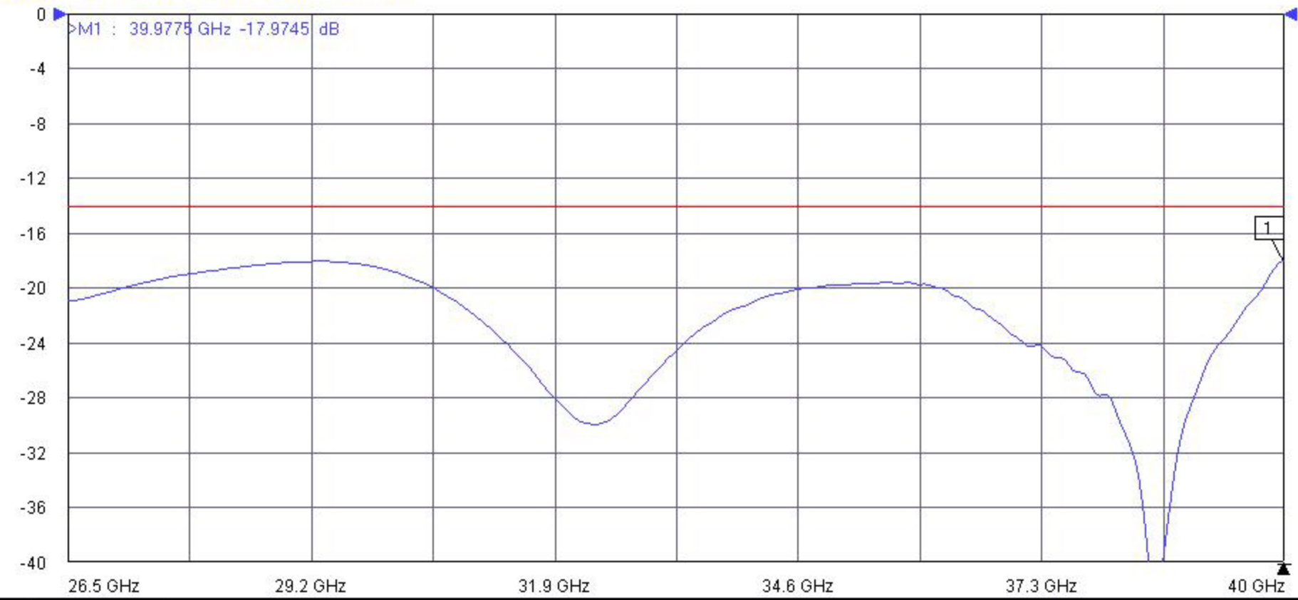
P1 VSWR S11 Refl LogM RefLvl: 0 dB Res: 4 dB/Div
