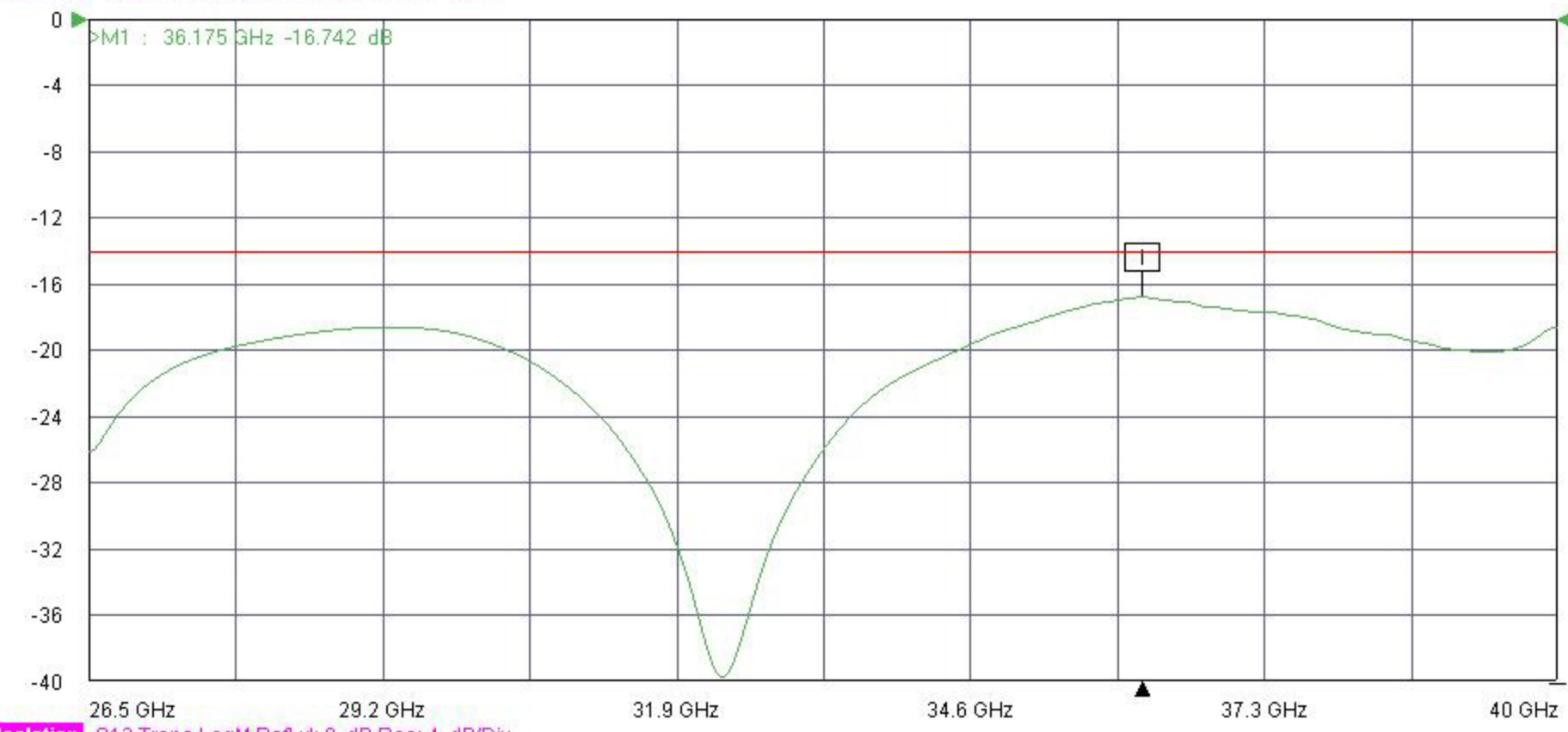
Isolation S12 Trans LogM RefLvl: 0 dB Res: 4 dB/Div
