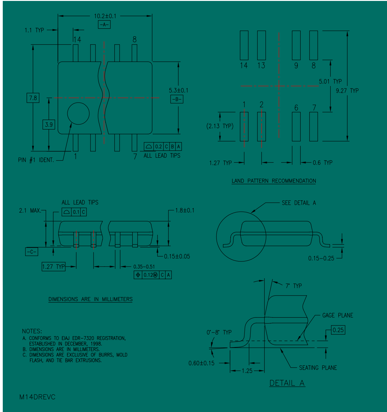
Figure 2. 14-Lead Small Outline Package (SOP), EIAJ TYPE II, 5.3mm Wide
