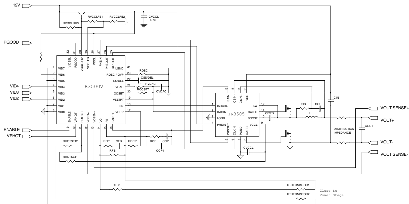
Figure 1 – Single Phase VR11.1 CPU VTT Application Circuit
