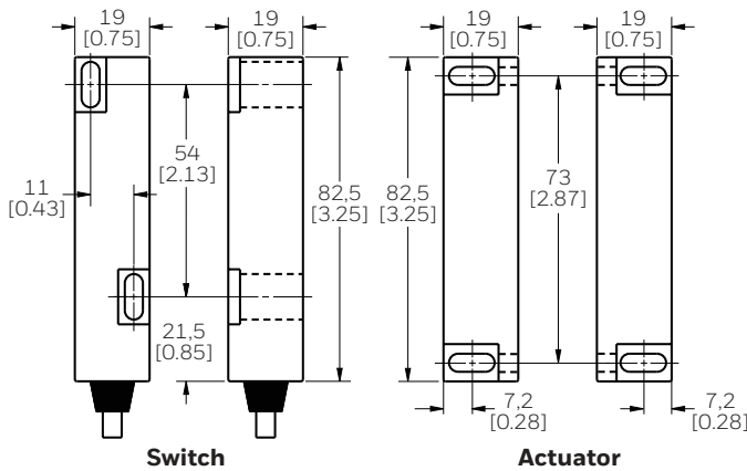
FIGURE 2. MOUNTING DIMENSIONS (FOR REFERENCE ONLY: mm [in])
