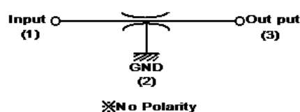
a)Equivalent Circuit
