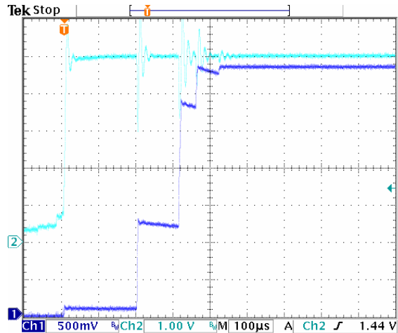
SUPPLY VOLTAGE, FAST TURN ON (TRISE = 1μS)
