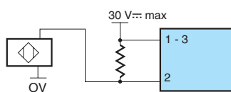
Start/Stop or reset input: 2-wire proximity sensor R=470 \Omega/2 \text{ W} for 2-wire leakage current detector \leq 1 \text{ mA}
