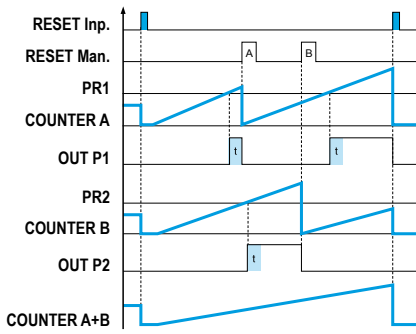
Output operation: OtoP MurS0 (AS)
