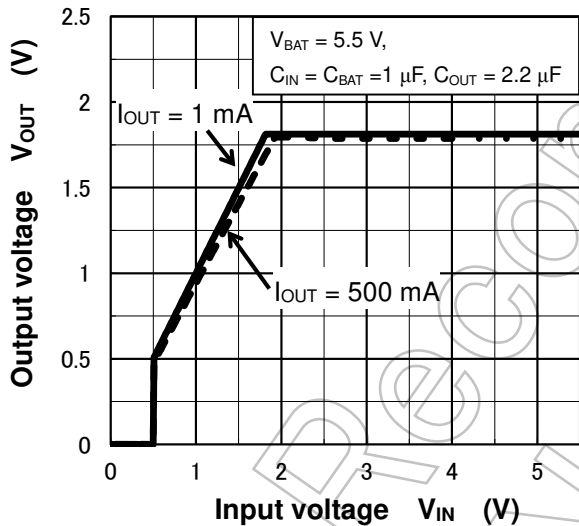
V_{OUT} = 1.8\text{ V}
