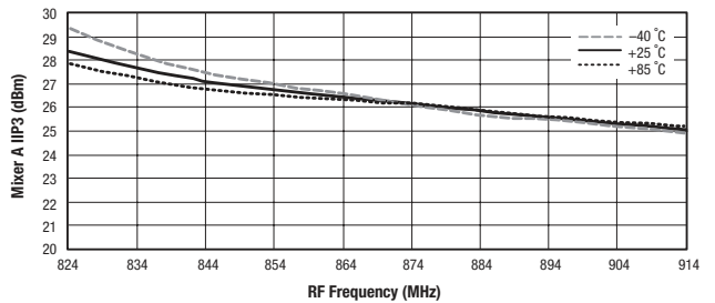
Figure 14. Mixer A IIP3 vs Frequency and Temperature
