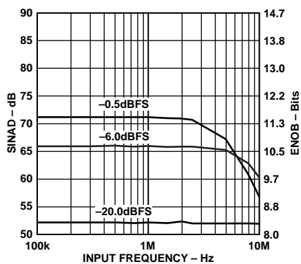
Figure 14. SINAD vs. Input Frequency (Input Span = 2 V, V_{CM} = 2.5 V)
