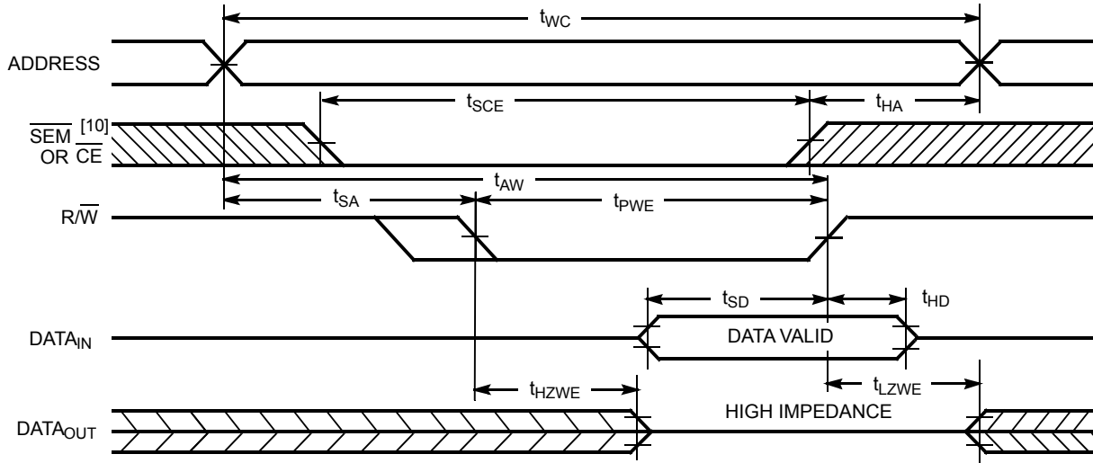
Write Cycle No. 2: \overline{R/W} Three-States Data I/Os (Either Port) [16, 18]
