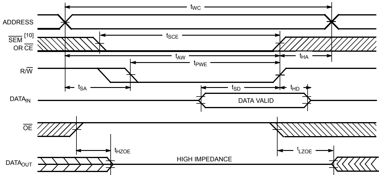
Write Cycle No. 2: \overline{R/W} Three-States Data I/Os (Either Port) [16, 18]
