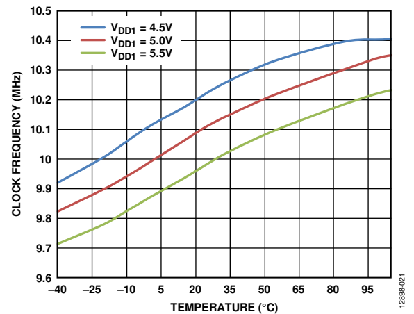
Figure 21. Clock Frequency vs. Temperature for Various Supply Voltages
