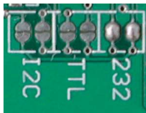
Figure 6: TTL Connections
