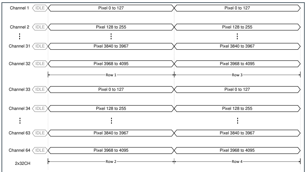
Figure 30: Pixel Mapping Using 2 \times 32 Channels
