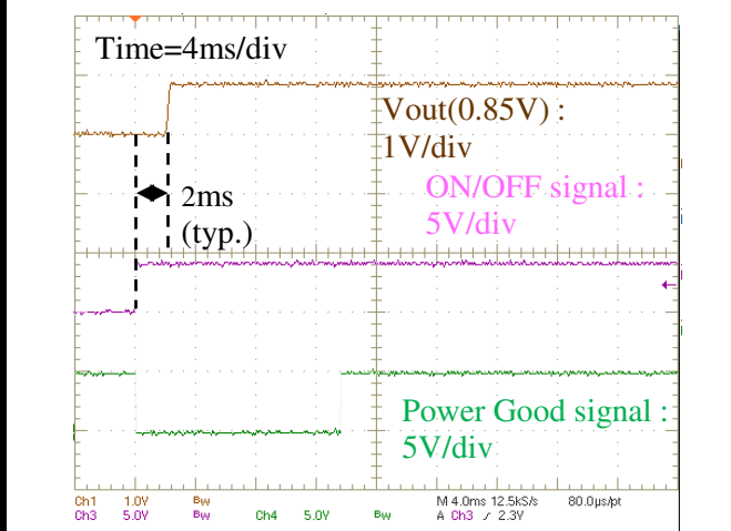
On/Off Enable Delay (Vin=5.0V, Vout=0.85V, lout=0A, Cload=110uF)
