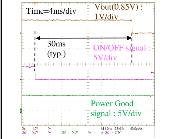
On/Off Enable Delay (Vin=5.0V, Vout=0.85V, lout=0A, Cload=110uF)
