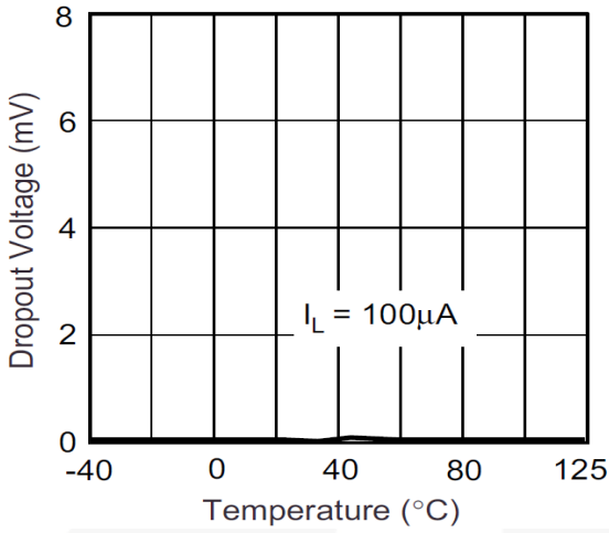
Figure 21. Dropout Voltage
