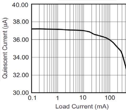
Figure 14. Ground Pin Current
