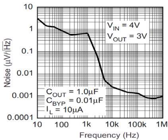
Figure 13. Noise Performance
