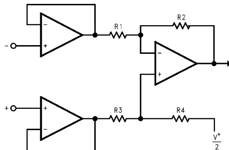
Figure 45. Three-op-amp Instrumentation Amplifier
