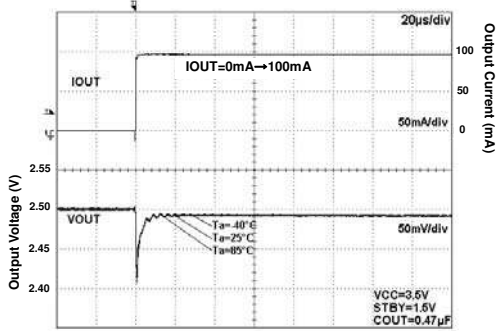
Fig 117. Load Response
