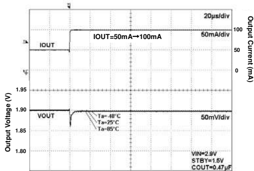
Fig 95. Load Response
