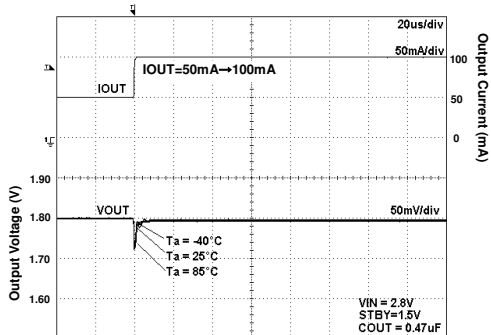
Fig 70. Load Response
