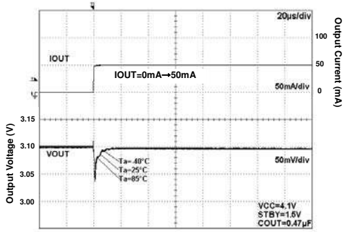
Fig 245. Load Response
