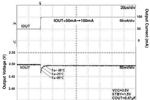
Fig 121. Load Response
