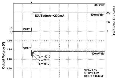
Fig 68. Load Response
