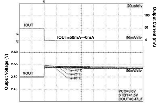
Fig 116. Load Response
