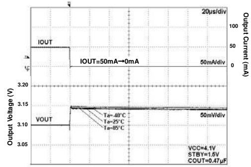
Fig 246. Load Response
