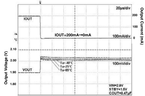
Fig 94. Load Response
