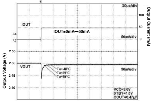
Fig 115. Load Response
