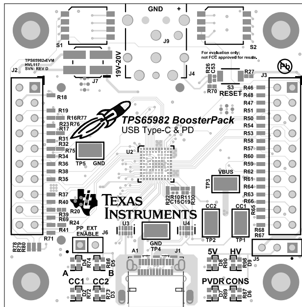
Figure 6. PCB Layer 1 (Component View)
