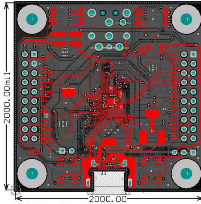
Figure 5. PCB Layer 1 (Top Layer)
