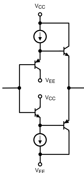
Figure 8. Output Stage
