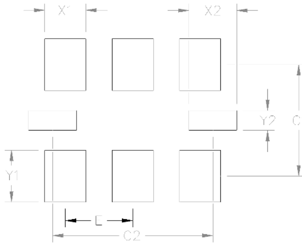
Figure 6.1. Si542 (5x7 mm) PCB Land Pattern
