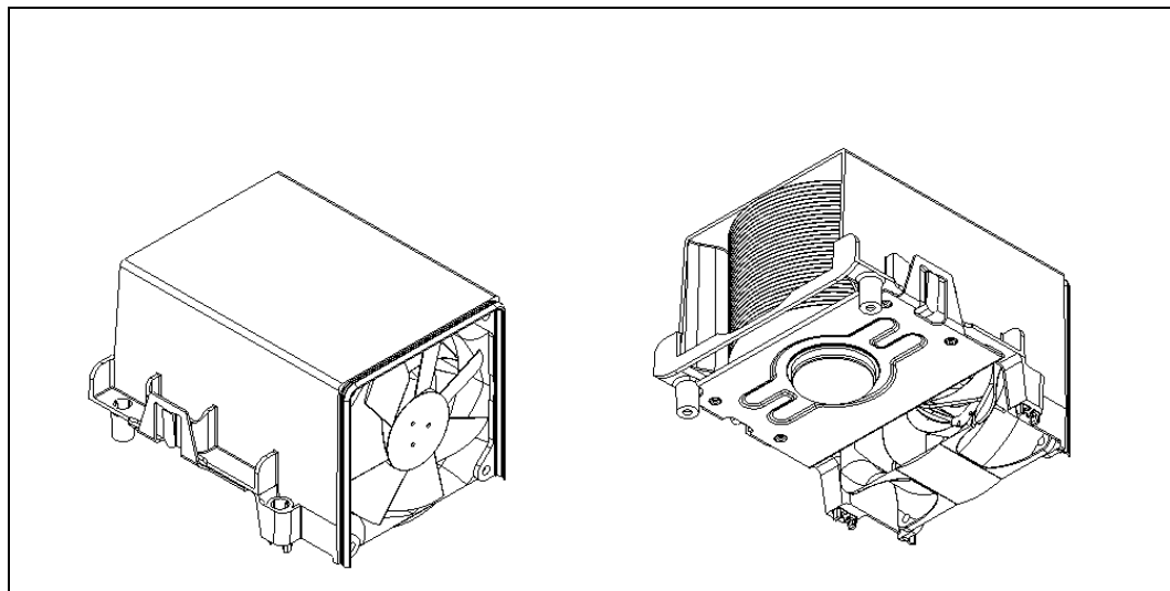
Figure 39. Mechanical Representation of the Boxed Processor with a Type I TMA
