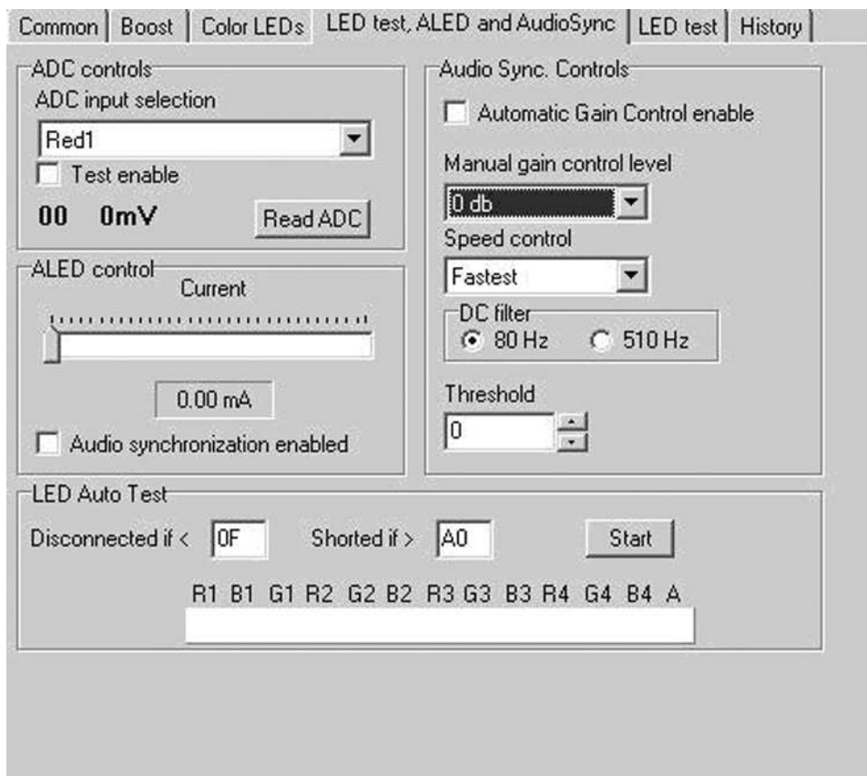
Figure 6. LED Test, ALED and Audio Sync Tab
