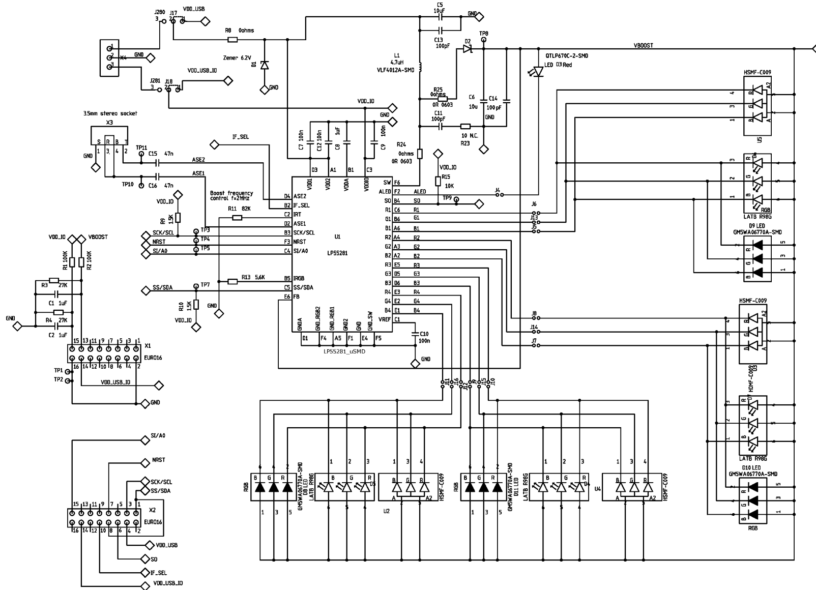
Figure 11. LP55281 Evaluation Board Schematic
