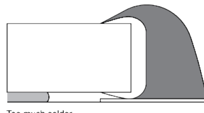
Too much solder Pad geometry too large, not soldered in preferred direction KKE0288-H-E
