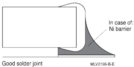
Good solder joint MLV0196-B-E
