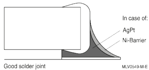
Good solder joint MLV0549-M-E
