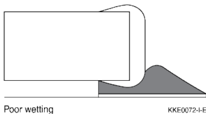
Poor wetting KKE0072-I-E
