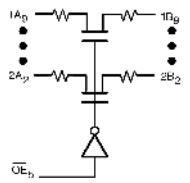
4-Bit Configuration
