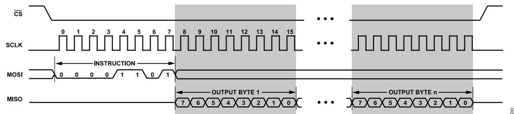
Figure 40. FIFO Read
