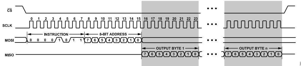
Figure 38. Burst Read
