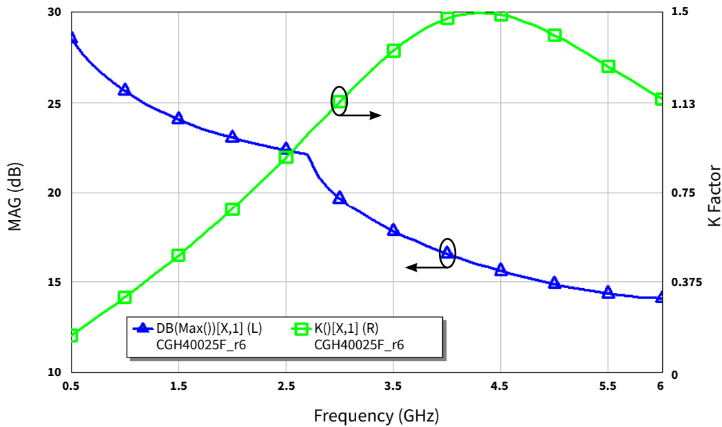
Figure 4. Maximum Available Gain and K Factor of the CGH40025 V_{DD} = 28\text{ V} , I_{DQ} = 250\text{ mA}
