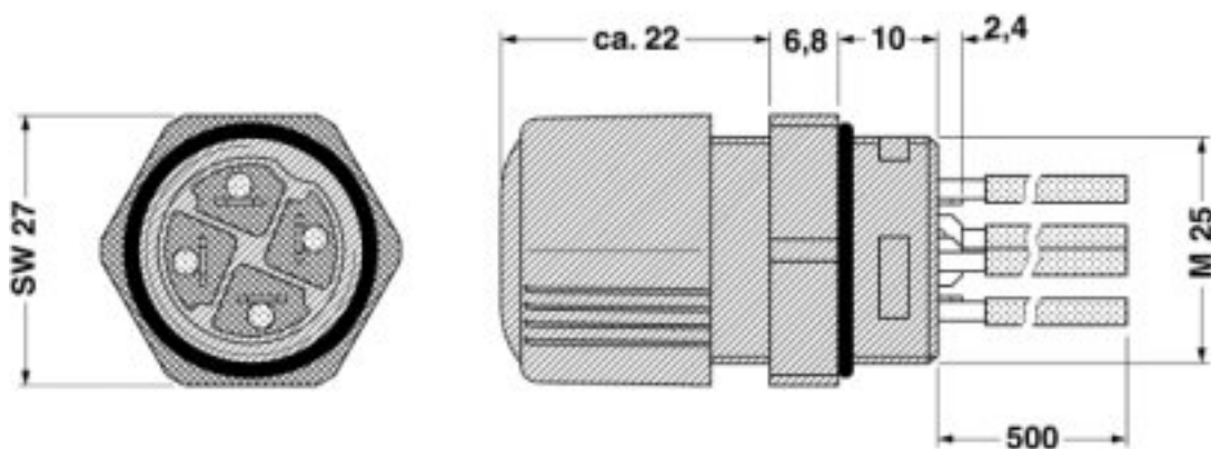
Dimensioned drawing
