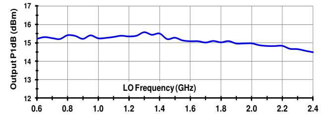
1dB Compression
