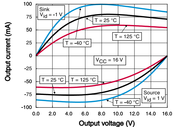
Figure 5. Output current vs. output voltage at V_{CC} = 16\text{ V}
