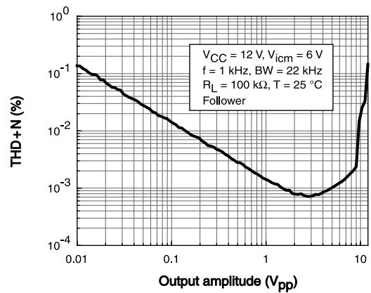
Figure 17. Distortion and noise vs. amplitude at V_{icm} = V_{CC}/2 and V_{CC} = 12\text{ V}
